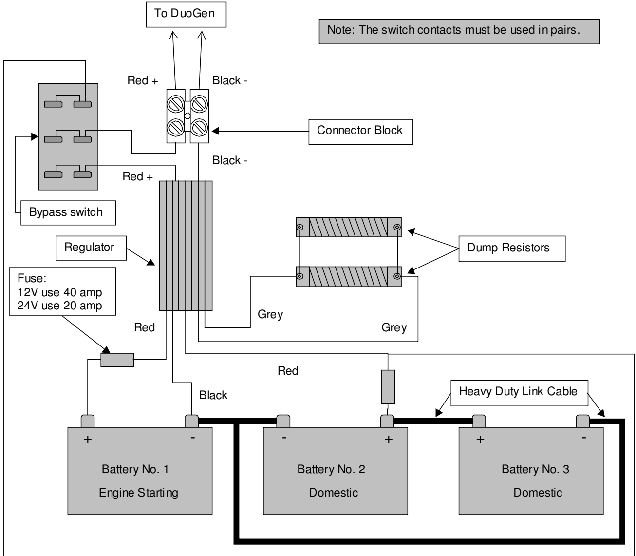
Domestic Batteries 2 & 3 are shown connected in parallel
